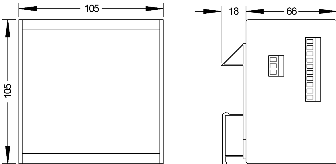
Dimensions TI125.x.x
